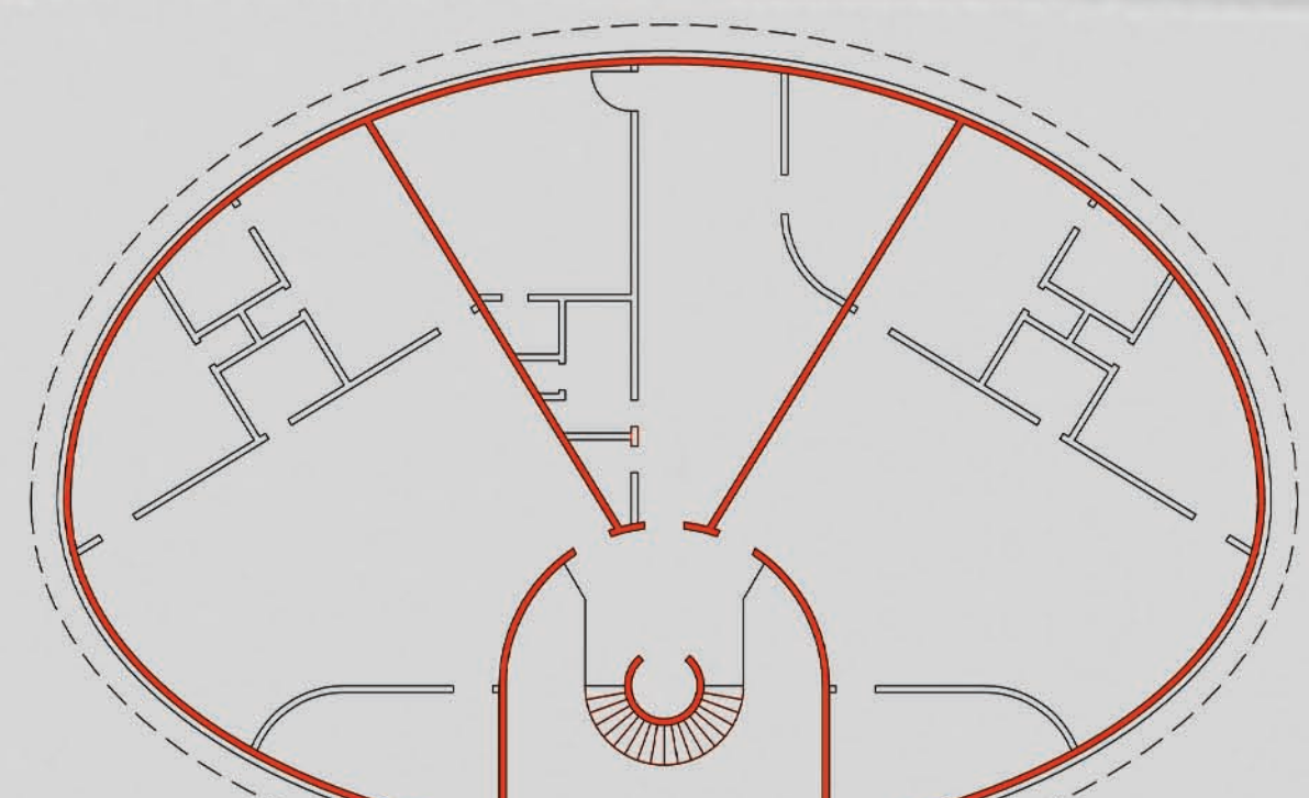
Structural Floor Plan 1"=16'
