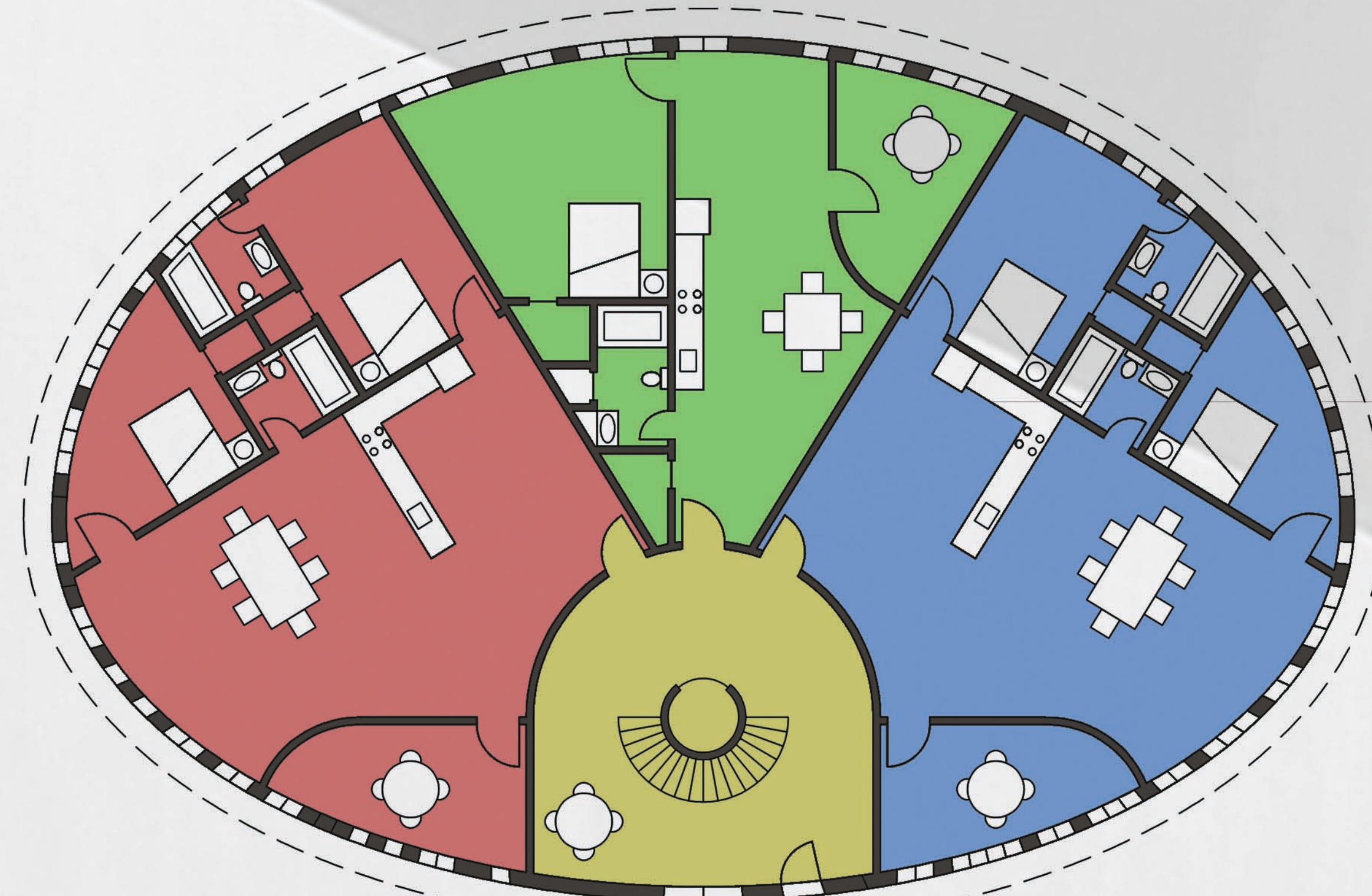
Lower Floor Plan 1"=8'
