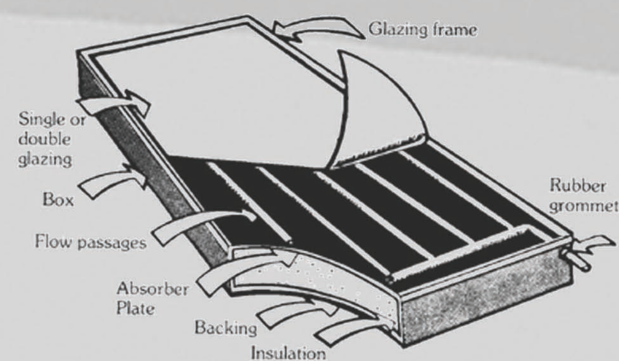
Solar Water Heating Detail
